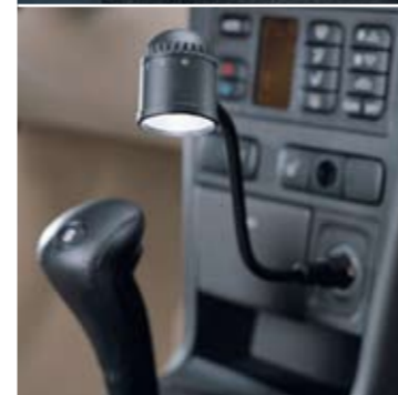
Reading lamp – with matt black finish, 20 cm flexible arm. Halogen bulb provides powerful light. Equipped with a universal connector, suitable for cars and caravans. Supplied with an adapter for plugging into the cigarette lighter socket.
