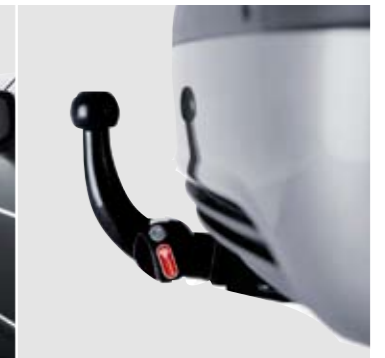
Towbar – choose between a fixed and an easily removed/lockable towbar. For fitting to the mounting points provided. Crash-tested. Some models require that a cutout is made in the bumper.
